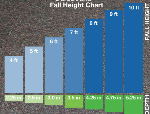
DuraBound™ Fall Height Chart
