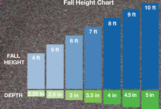
DuraBound™ Fall Height Chart
